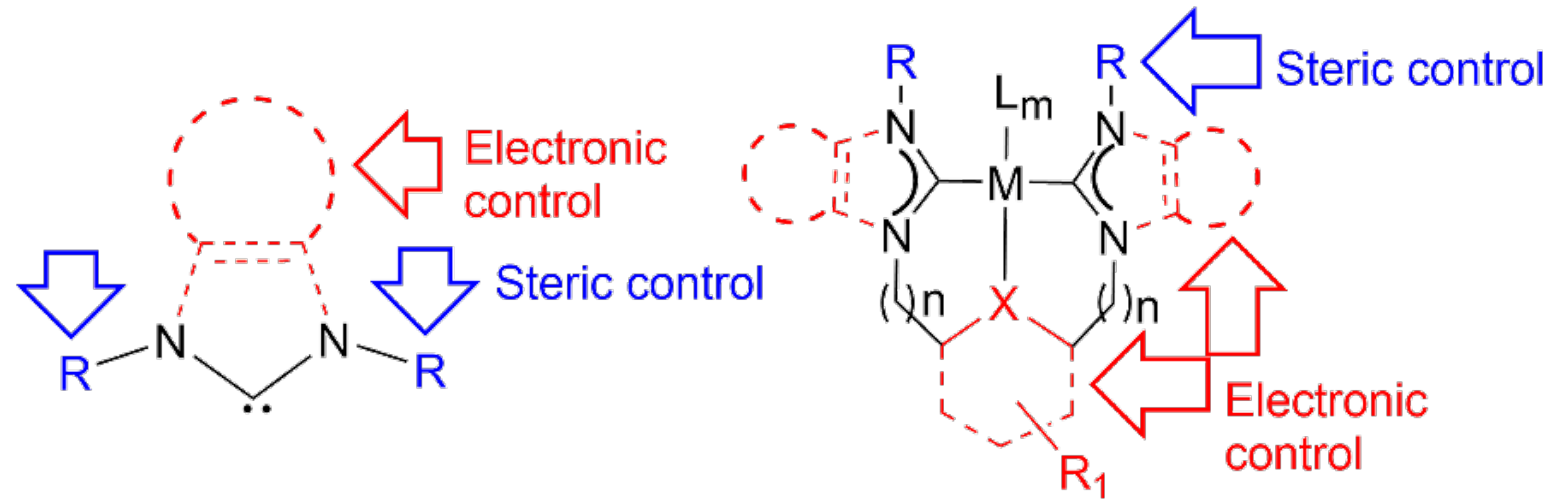
a) NHC and b) metal complex with a pincer type bis-NHC ligand.
